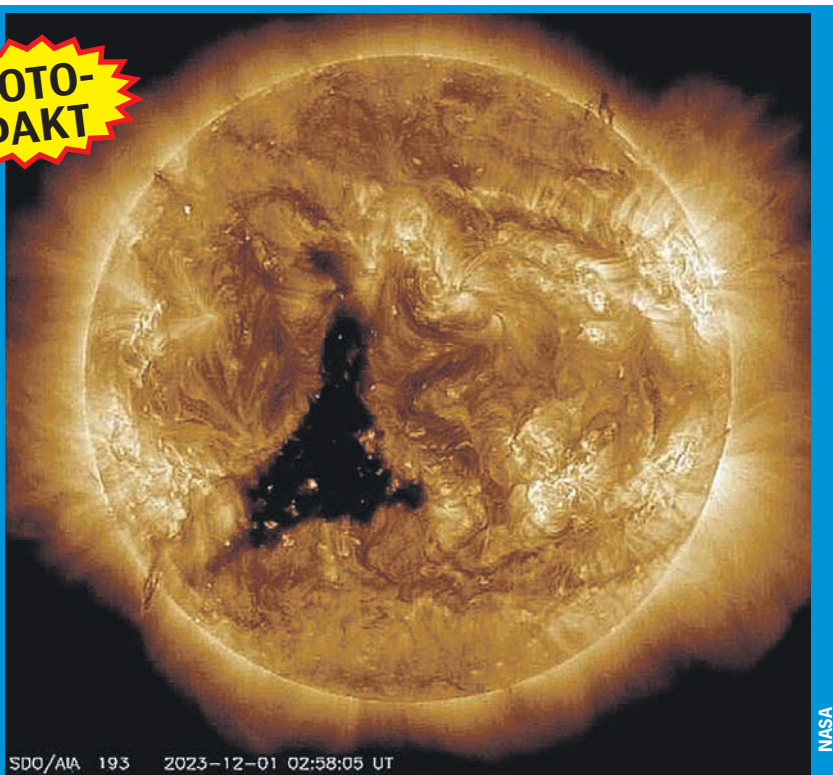
SDO/AIA 193 2023-12-01 02:58:05 UT
